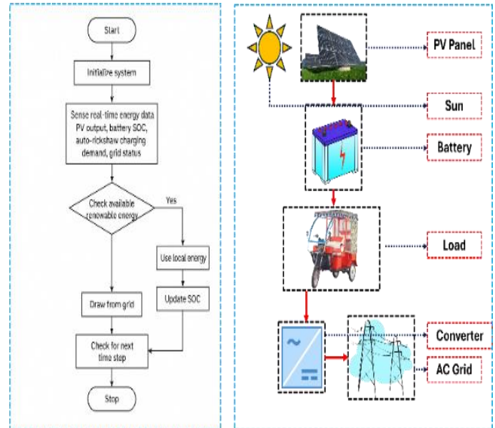
Fig. 2. Conceptual flow chart and block diagram of the system
