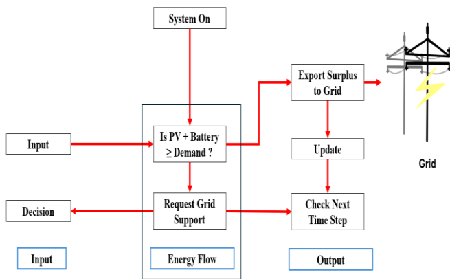
Fig. 3. Energy sharing model flowchart
